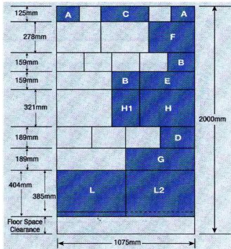
(Floor space clearance variable in different configurations)
